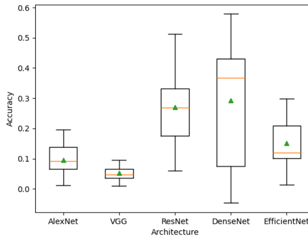
Box plot
