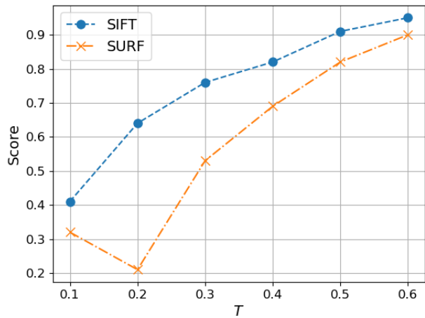
Line chart
